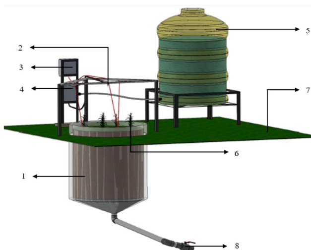
1 – lysimeter, 2 – irrigation nozzle, 3 – soil moisture sensors and pump control panel, 4 – pump, 5 – reservoir, 6 – plant, 7 – soil surface
