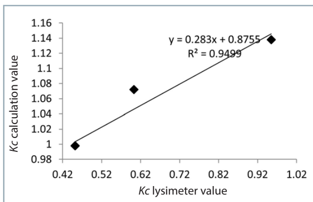
Fig. 5 The correlation of Kc values
