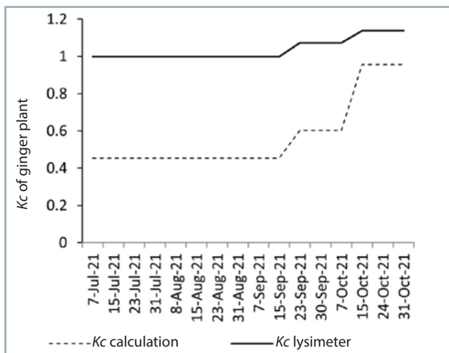
Fig. 4 Kc of ginger plant
